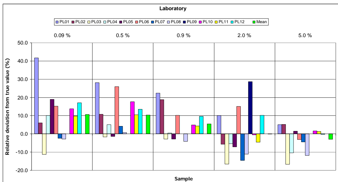
Figure 1. Relative deviation (%) from the true value of DP-356043-5 for all laboratories
